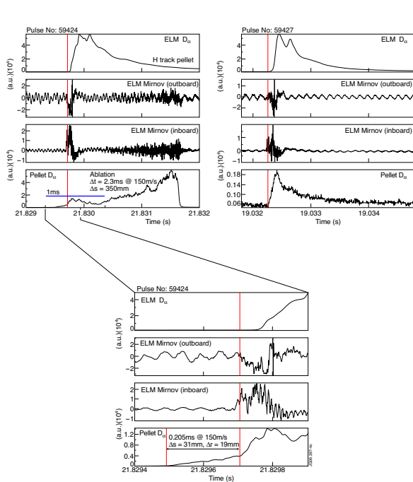
Figure 3: Upper: Comparison of triggered (left) and intrinsic (right) ELM. Signals from top: D_\alpha outer divertor, MHD outboard and inboard ELM monitors, ablation monitor. Lower: expansion of ablation and ELM onset for triggered ELM.
