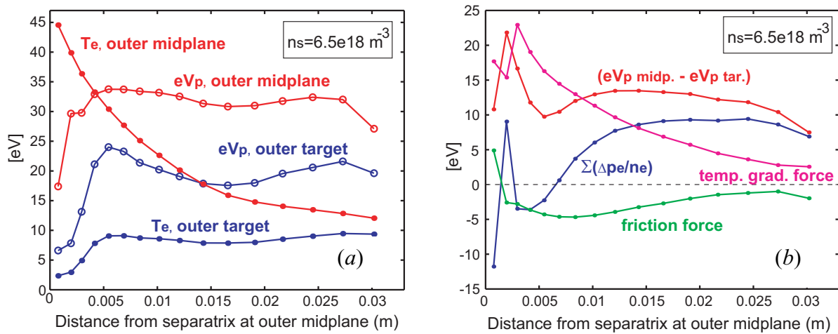
Fig. 1. T_e and plasma potential V_p (multiplied by elementary charge e ) at the outer midplane, T_e and eV_p at the outer target (a); the difference between outer midplane and outer target eV_p , and its contributions: integrated friction force e j_{||}/\sigma_{||} , integrated temperature gradient force \approx -0.71 \nabla_{||} T_e , and integrated pressure gradient force -\nabla_{||} p_e/n_e (marked as \Sigma(\Delta p_e/n_e) (b), for Ohmic JET case with n_s = 6.5 \times 10^{18} m^{-3} . The distance from the separatrix is mapped to the outer midplane position.
