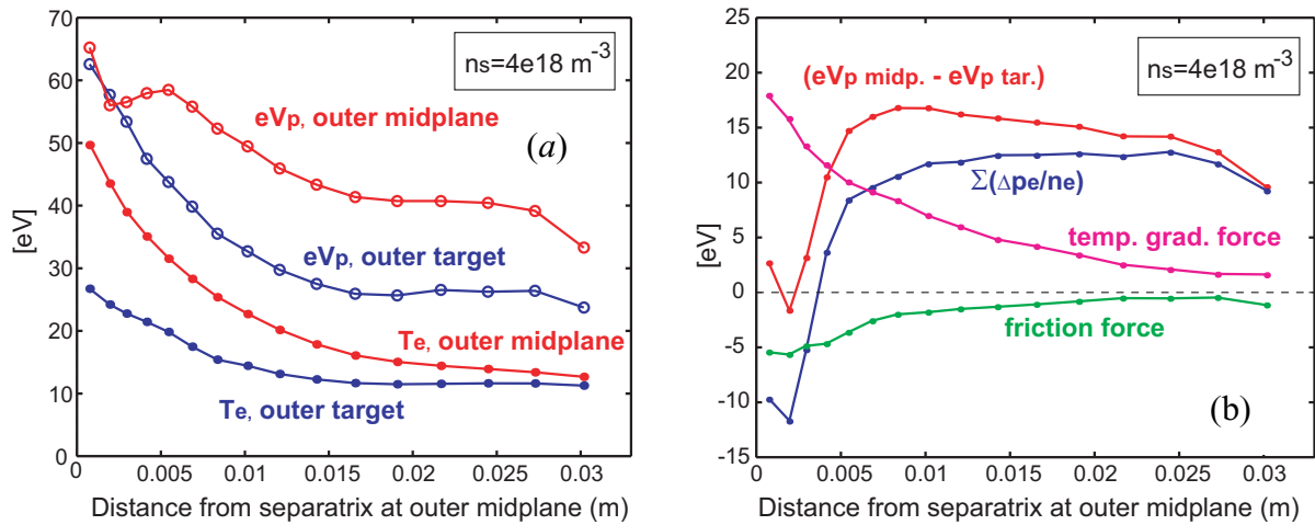
Fig. 2. Same data as shown in Fig. 1, but for the lower density Ohmic case, with n_s = 4 \times 10^{18} m^{-3} .
