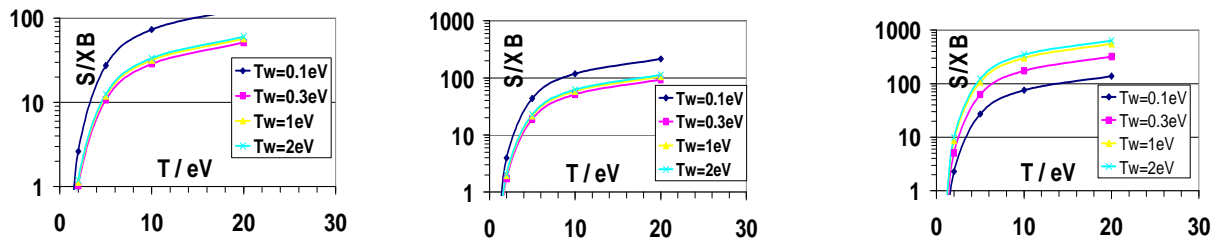
Fig.1: S/XB for 4008.75 Å for 4294.61 Å for 5053.28 Å displayed in fig.1 for 3 selected lines. Values for more lines will be found in a forthcoming paper [7]. The influence of the value for T_W can be intensively studied for the 2551 Å, 5053 Å and 4982 Å lines as these are excited from the lowest configurations of the ground state ( ^5D_{0,1} ) which are continuously depopulated for increasing T_W .
