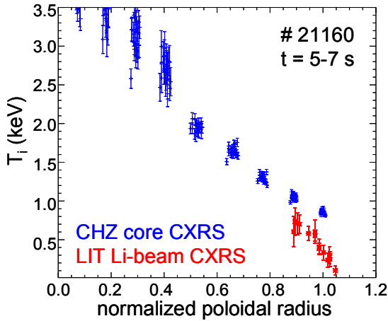
Figure 1: Measured ion temperature profile for shot #21160, t=5-7 s. The blue data points are from the core CXRS diagnostic, the red points from Li-beam CXRS edge diagnostic.
