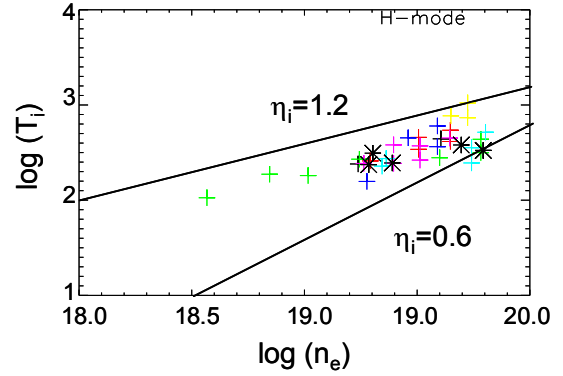
Figure 2: Double logarithmic plot of T_i vs n_e for 6 different H-mode discharges. Only data in the ETB, 0.96 < \rho_{pol} < 1.01 are taken. The solid lines show gradients of 0.6 and 1.2 to guide the eye to the values determined as minimum and maximum for \eta_i .
