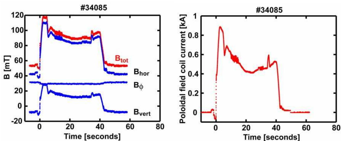
Fig. 2: Left panel - 3D Hall record of the shot #34085 with the maximum plasma current of 640 kA. Measured components of the magnetic field B_{\phi} , B_{hor} , and B_{vert} are plotted by blue, while the computed amplitude of the total magnetic field at the probe location is plotted by red. The right panel shows the current flowing through the poloidal field coil.
