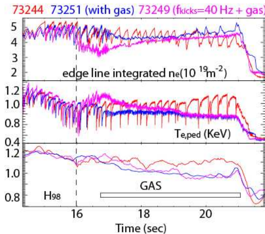
Fig. 3: Temporal evolution of pedestal T_e and n_e (line integrated) and H_{98} factor for three pulses: 73244(unfuelled), 73251(with gas fuelling), 73249 (with gas fuelling and 40 Hz kick starting at 16 sec); showing the plasma response to gas
