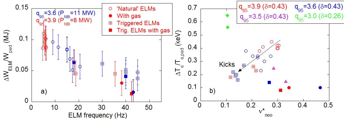
Fig.4: a) Normalized ELM energy loss (to the pedestal energy) versus ELM frequency, b) Normalized electron temperature perturbation caused by the ELMs versus pedestal plasma collisionality showing that, with kicks, small ELMs can be sustained even at low pedestal collisionality.
