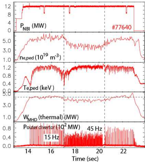
Fig. 1 Temporal evolution of the pedestal top electron density and temperature, thermal W_{MHD} and heat flux from fast IR measurements. Kicks at 45 Hz are applied between 17 and 20 sec.
