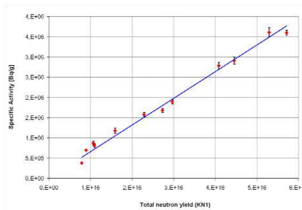
Fig. 1. Specific activity of Y-89m measured by means of HPGe detector vs total neutron yield.
