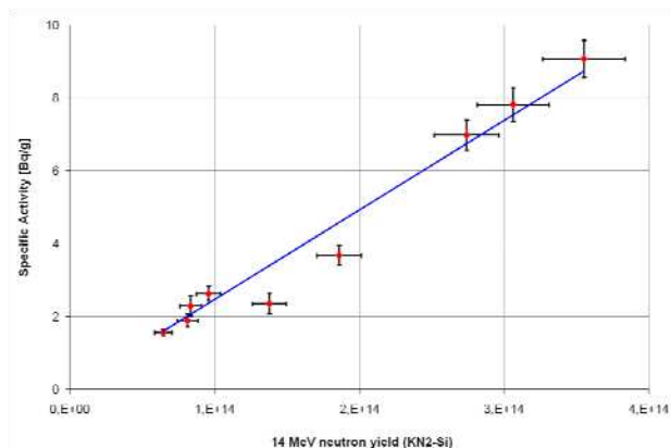
Fig. 2. Specific activity of Mn-56 from cobalt sample vs 14 MeV neutron yield.
