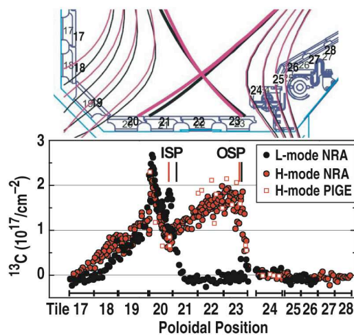
Fig 1. ^{13}\text{C} measured in divertor by NRA and PIGE.
