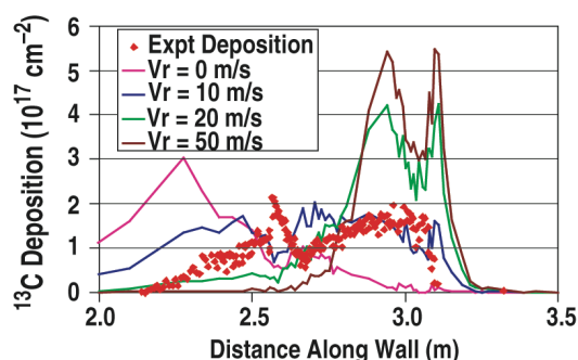
Fig. 3. OEDGE code analysis showing the influence of a radial pinch on the ^{13}\text{C} deposition pattern. Fast parallel plasma flow along the inner SOL has also been included here, at M = 0.3 (Fig. 4). Modeling assumes time-invariant plasma conditions; see [4].
