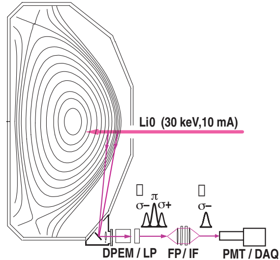
Fig. 1. Diagnostic layout. The 670 nm resonance fluorescence light from the collisionally excited beam is imaged at a series of closely spaced locations in the plasma edge. The polarization state of the \sigma -Zeeman sublevel is analyzed by passing the light through dual photoelastic modulators (DPEM) and a linear polarizer (LP) to amplitude modulate the emission, which is detected by a bank of 32 photomultiplier tubes (PMT). Individually tuned etalon pairs (FP) and an interference filter (IF) isolate the \sigma -component for each of the Doppler-shifted viewing locations. Lock-in analysis identifies the ratio of circular to linear polarization and, in conjunction with a spatial calibration, determines the value of the poloidal field at each measurement location.
