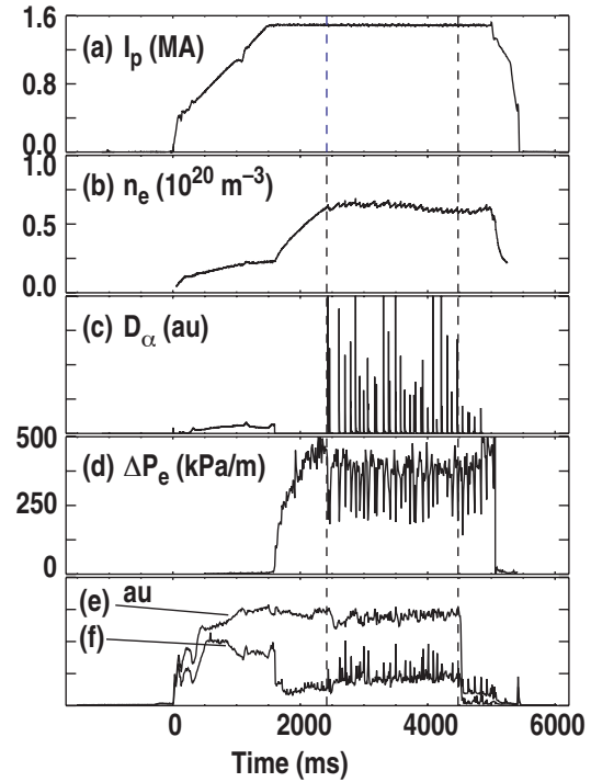
Fig. 2. Time traces for DIII-D shot 119089. (a) Plasma current I_p , (b) plasma density n_e , (c) divertor D_\alpha , (d) edge pressure gradient \Delta P_e from Thomson scattering, (e) lithium fluorescence at top of pedestal, (f) lithium fluorescence at foot of pedestal. ELMing period from 2400 to 4450 ms is used in subsequent analysis.
