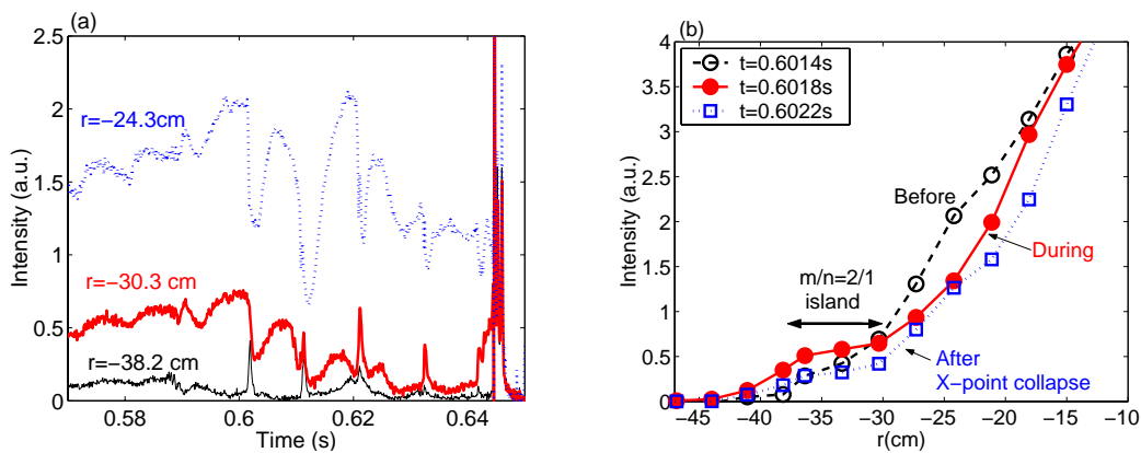
Figure 1 (a) Time evolution of line-integrated x-ray emission near the q=2 surface and (b) radial profiles of x-ray emission measured by a soft x-ray camera viewing the high field side of plasma.
