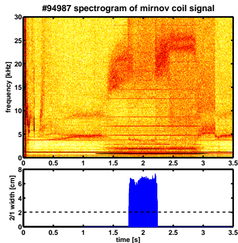
Figure 5: Spectrogram of magnetic signal and 2/1 island obtained from SXR, showing, that the Alfvén waves can be excited by the external perturbation field without 2/1 tearing mode. Contradictory to earlier publications, the 2/1 tearing mode even suppresses the Alfvén waves at t = 1.8 s, destabilized again when the tearing mode is stabilized t = 2.25 s.
