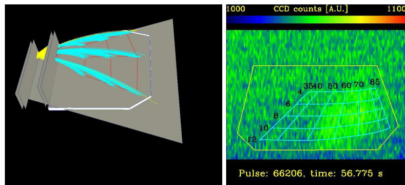
Figure 1: Left: 3D visualisation of particle orbits with JET probe geometry resulting in a sample 3x3 grid (red). Yellow particle orbits are discarded. Right: Emission pattern overlaid with 5x6 grid covering the accessible phase-space.
