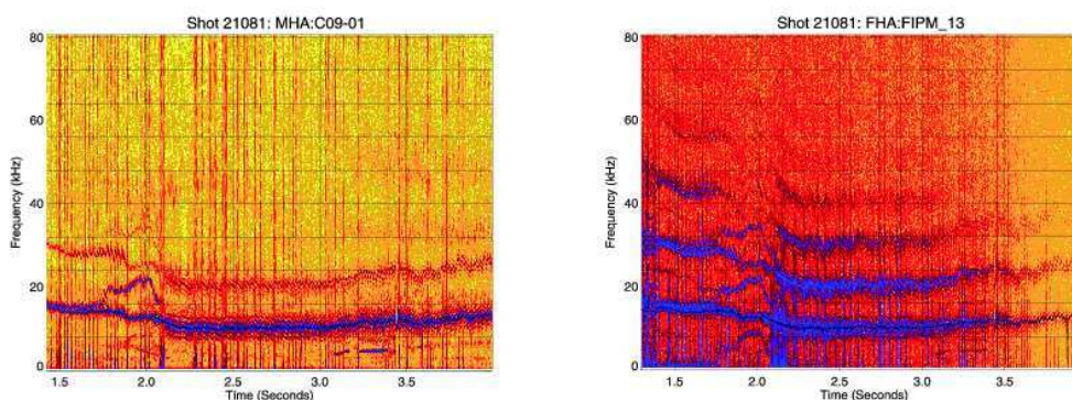
Figure 4: Time evolution analysis of the frequency of a (3,2) NTM magnetic perturbation, \dot{B}_\theta , on the left and a FILD channel on the right
