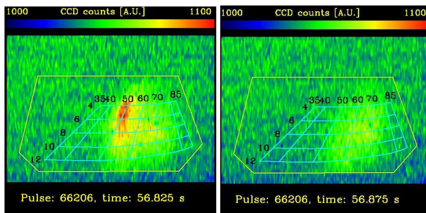
Figure 2: CCD camera images (Units: counts) with phase-space mapping of consecutive times of JET #66206 illustrating the additional losses due to sawtooth activity (during the exposure time lasting from 56.80 s - 56.85 s). The image sequence is representative of all monster sawtooth induced particle losses observed so far.
