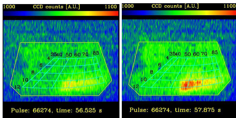
Figure 3: Pulse #66274 which was heated with 16 MW of NBI power. After 57.0 s, 3.3 MW of ICR heating have been added. The left image shows the loss products widespread in pitch angle but narrow in energy. With added ICRH some more particles are lost, but seem to be somewhat more localised in pitch angle ( \approx 50^\circ ).
