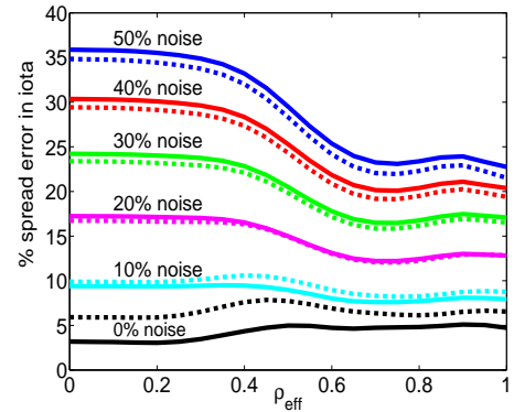
Figure 1: Error profiles of iota recovery for different noise levels. Solid line: c-FP model; Dashed line: q-FP model.
