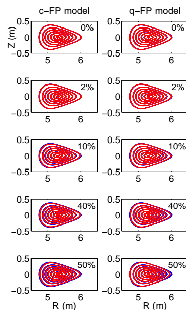
Figure 4: Flux surface recovery in the triangular plane. Quoted are percentage noise on J(s) . Blue: VMEC surfaces; Red: FP-recovered surfaces.
