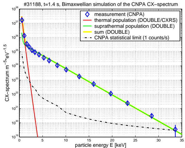
Figure 8: Compact NPA CX spectrum and DOUBLE simulation. n_i^{(1)}/n_i^{(0)} = 0.1 , T_i^{(0)} = 300 eV, T_i^{(1)} = 2.4 keV, E_{knee} = 1.6 keV.
