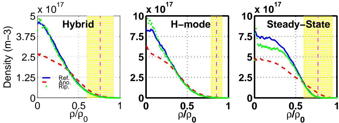
Figure 2: Alpha particle density profiles for f_{LH} = 3.7 GHz, for the three ITER scenarios: without ripple nor anomalous transport (reference, in blue); with magnetic field ripple only (in green), and with anomalous transport only (with D_{ano}^{rr} = 1\text{m}^2/\text{s} , in red) The colored area represents the region where LH power is absorbed by alpha particles.
