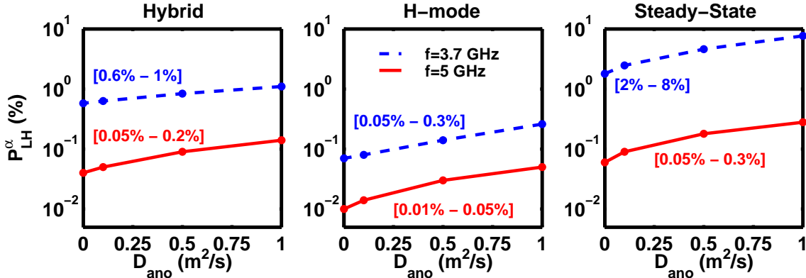
Figure 3: LH power absorbed by alpha particles as a function of the anomalous diffusion coefficient, for the three ITER scenarios, both for f_{LH} = 3.7 and 5 GHz (without magnetic field ripple).
