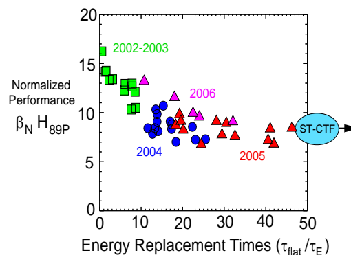
Figure 1 – Product of normalized beta and H-mode confinement enhancement factor relative to ITER-89P scaling vs. flat-top duration normalized to energy confinement time.
