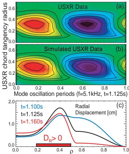
Figure 4 - Measured line-integrated USXR emission amplitude contours plotted versus chord tangency radius and time for one oscillation period, (b) best-fit simulated USXR emission amplitude assuming a 1/1 kink eigenfunction, and (c) reconstructed kink radial displacement amplitude profile at outboard midplane during mode saturation.
