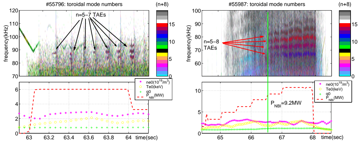
Figure 3a. Limiter plasma: n=5\div 7 TAEs unstable at P_{NBI}=6MW , |\nu_{\parallel}|\approx 0.8\nu_A . Figure 3b. X-point plasma: n=5\div 8 TAEs unstable at P_{NBI}=9.2MW , |\nu_{\parallel}|\approx 0.95\nu_A .
