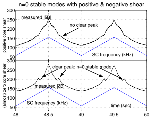
Figure 5. Amplitude of stable n=0 modes for two discharges with monotonic q -profile and positive core magnetic shear (top) and non-monotonic q -profile with almost zero core magnetic shear (bottom).
