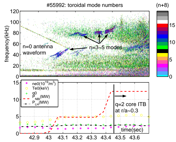
Figure 4b. Unstable n=3\div 5 modes.
