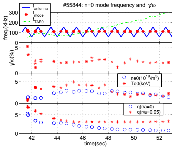
Figure 4a. Weakly damped n=0 modes.
