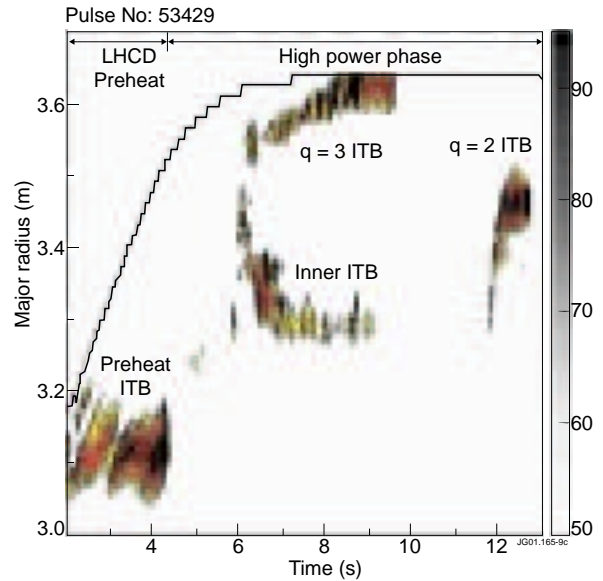
Figure 4. The contours of constant \rho^*_{Te} = \rho_s/L_{Te} \geq 0.01 [10] show the evolution of T_e ITB on shot 53429. LHCD preheat is from 1 to 4.4s, main heating starts at 4.4s, LHCD is reapplied at 5.7s.
