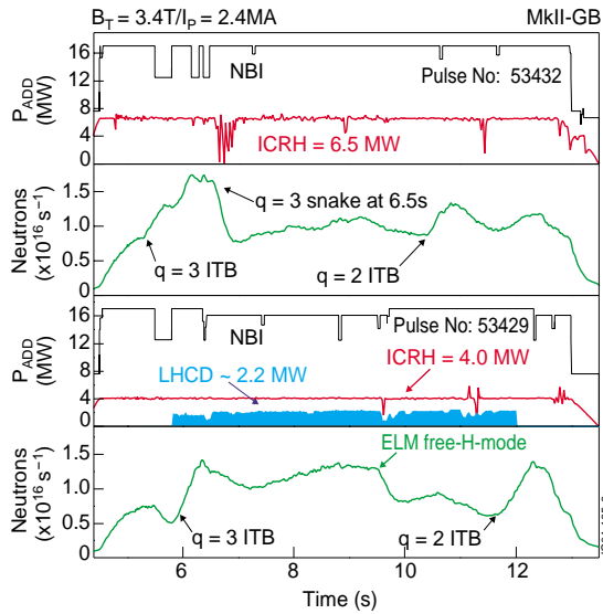
Figure 3. Additional heating power and neutrons for shot 53432 and 53429 (with LHCD during main heating). Both shots have LHCD preheat.
