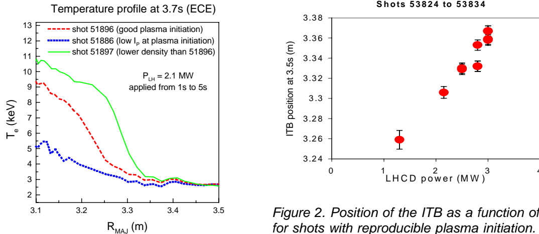
Figure 1. T_e profile during LHCD preheat for shots with different plasma parameters.
