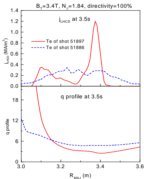
Figure 5.a) j_{LHCD} , and b) q profiles, during preheat for shots with and without electron transport ITB.
