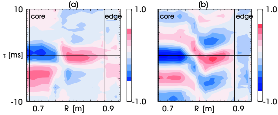
Figure 3: Cross correlation between a core PCI channel (17) and GPC2 vs R for HQA (left) and LQA (right). A positive time lag \tau means that PCI fluctuations occur before ECE changes. The time resolution is 0.5 ms.
