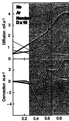
Figure 5: Comparison between Ar and Ne transport coefficient for hybrid scenarios: three regions with different transport can be seen in the convection. The neoclassical values are shown in dashed lines.
