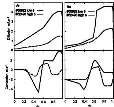
Figure 7: V and D dependence on triangularity: A change from outward to inward convection is seen in the edge region for both Ne and Ar.
