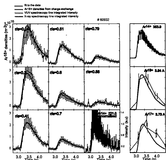
Figure 2: Argon modelled densities and line Intensities against CXRS, VUV and X-ray measurements.
