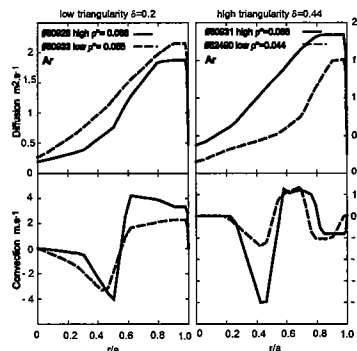
Figure 6: D and V dependence with \rho^* at constant q_{95} : Argon transport coefficients are plotted for each triangularity for low and high \rho^* .
