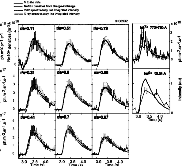
Figure 3: Neon modelled densities and line Intensities against CXRS, VUV and X-ray measurements.
