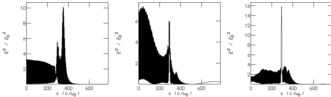
FIG. 2: Oscillations of the transverse electromagnetic field energy (left to right) for times 5.25, 5.5, 6 ps, the left plasma boundary is at 250 c/\omega_0 and the cavity position is at 290 c/\omega_0 .
