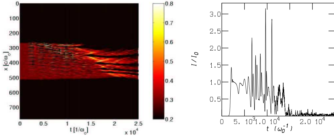
FIG. 1: Time evolution of the density in units of the critical density (left) and temporal variation of the backscattered intensity with respect to the incident laser intensity (right).
